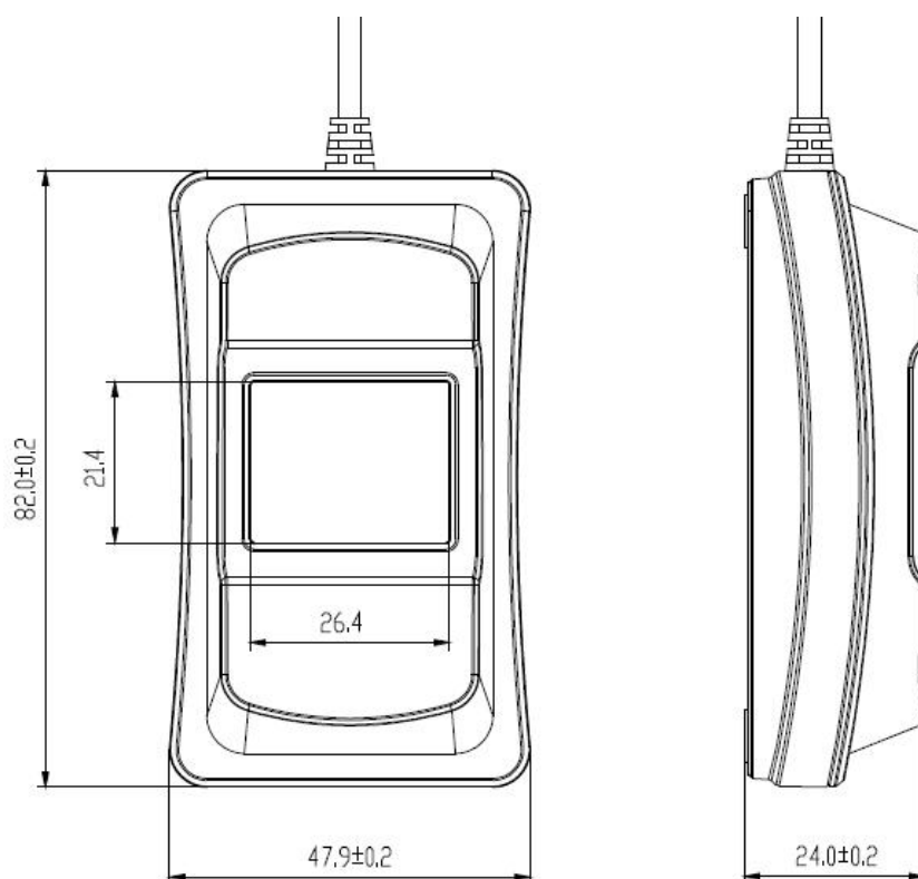
Mechanical Dimension (Unit: mm)
