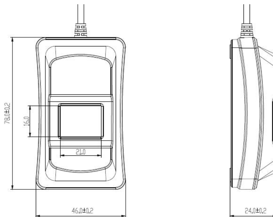
Mechanical Dimension (Unit: mm)
